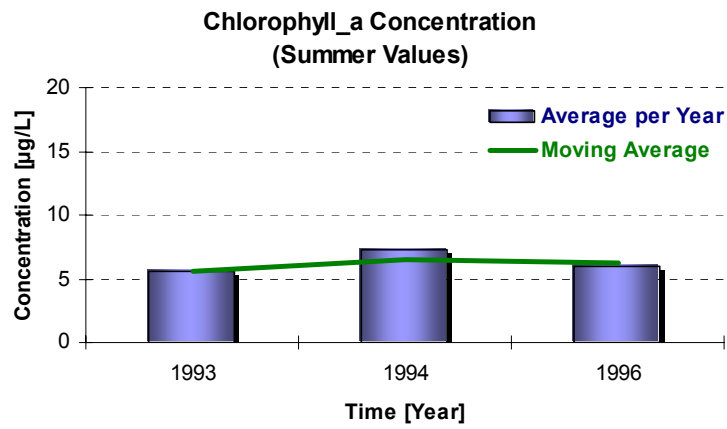
Figure 7 – Distribution of Chlorophyll-a Concentration during the summer
