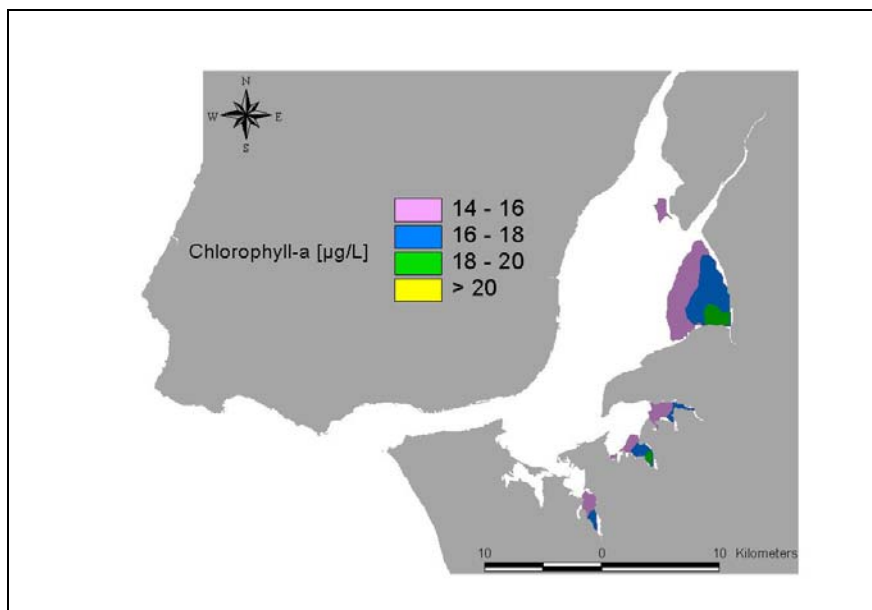
Figure 20 - Areas with Chlorophyll-a concentration above the Elevated Value (>14 \mu\text{g/L} )
