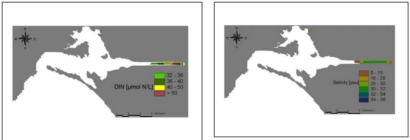
Figure 26 - Areas with DIN concentration above the Elevated Value ( >32 \mu\text{mol N/L} ); Spatial distribution of salinity
