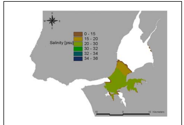
Figure 14 - Areas with DIN concentration between the Background and the Elevated Value (34-51 µmol N/L); Spatial distribution of salinity
