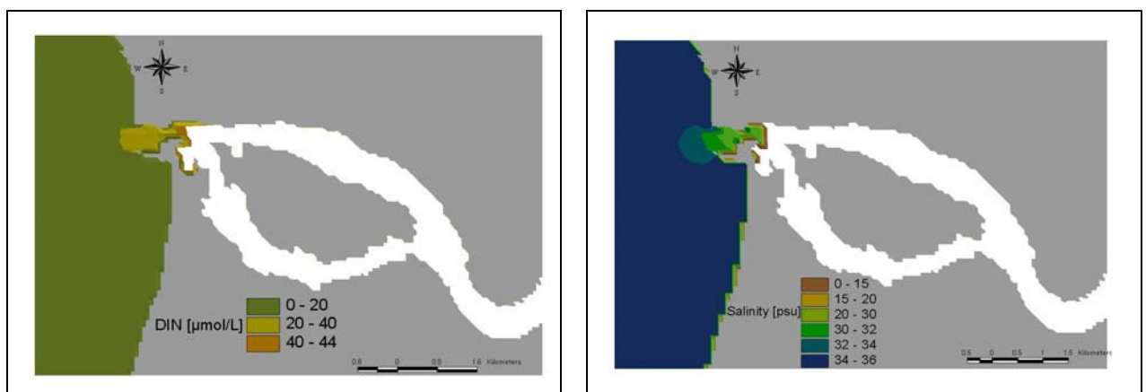
Figure 3 – Areas with DIN concentration below Background Value (0-44 \mu\text{mol N/L} ); Spatial distribution of salinity
