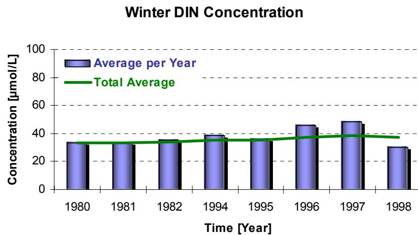
Figure 12 – Distribution of Winter DIN Concentration
