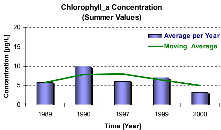
Figure 28 – Distribution of Chlorophyll-a Concentration during the summer
