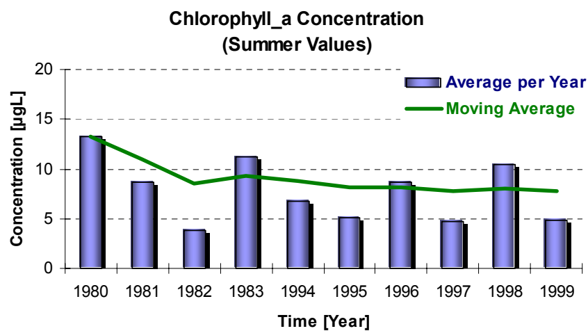
Figure 17 – Distribution of Chlorophyll-a Concentration during the summer
