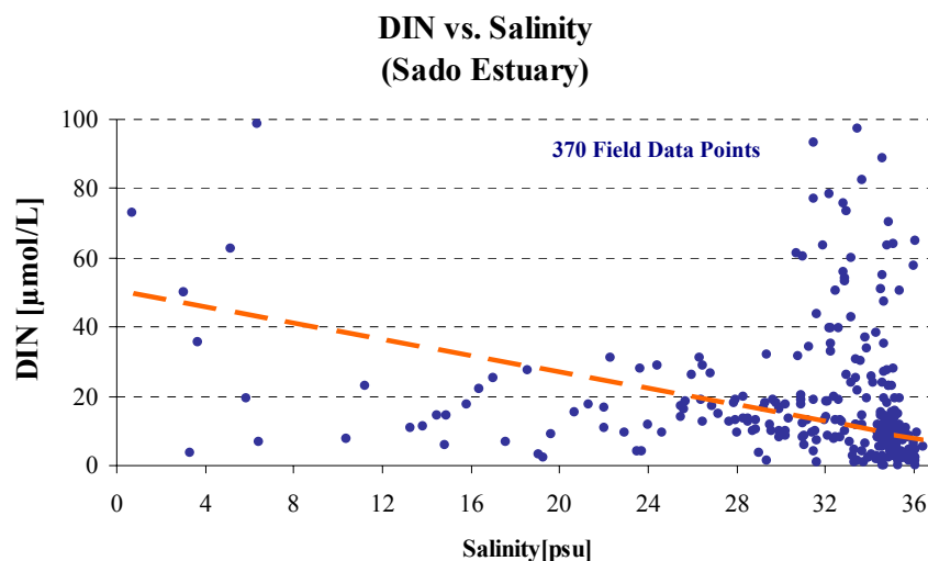
Figure 27 – DIN distribution vs. Salinity in Sado Estuary
