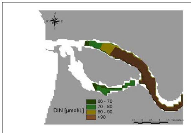
Figure 5 - Areas with DIN concentration above the Elevated Value (>66 \mu\text{mol N/L} ); Spatial distribution of salinity
