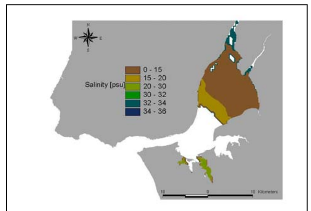
Figure 15 - Areas with DIN concentration above the Elevated Value (>51 µmol N/L); Spatial distribution of salinity
