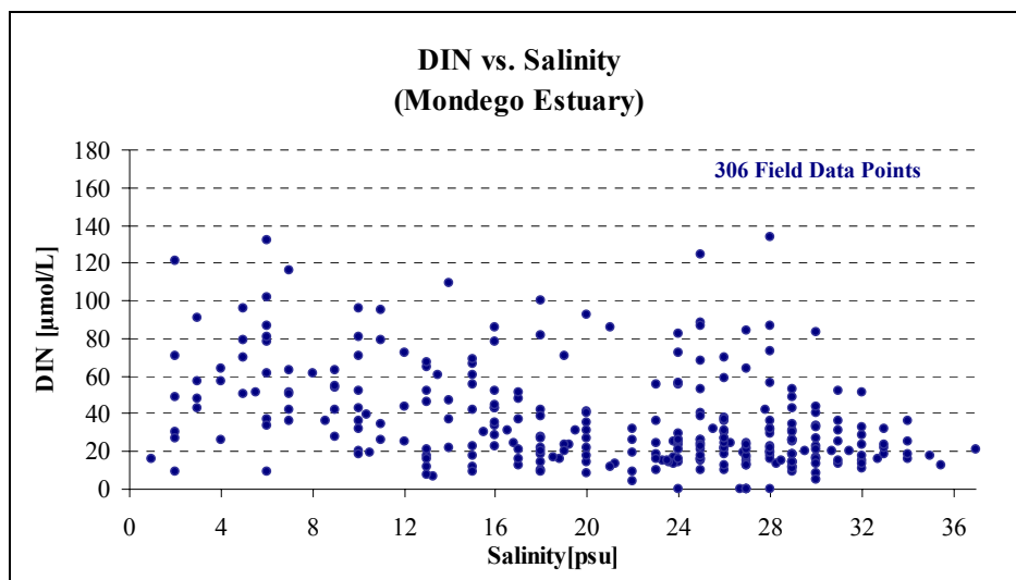
Figure 6 – DIN distribution vs. Salinity in Mondego Estuary
