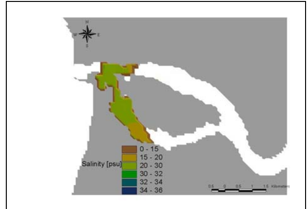
Figure 4 - Areas with DIN concentration between the Background and the Elevated Value (44-66 \mu\text{mol N/L} ); Spatial distribution of salinity
