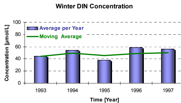
Figure 2 – Distribution of Winter DIN Concentration in the Mondego Estuary
